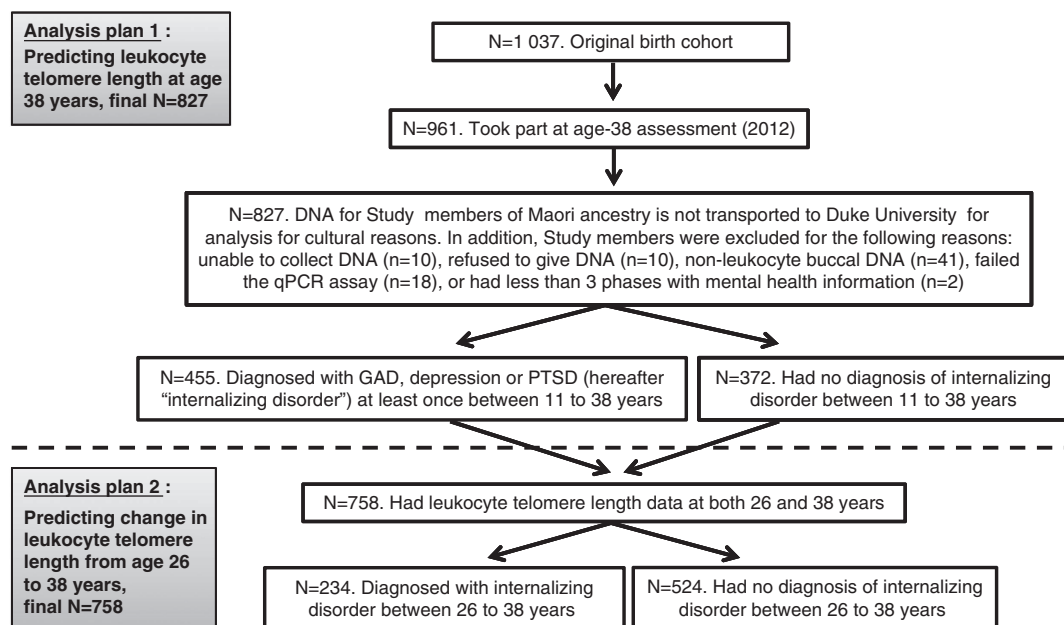
Figure 1. Analysis plan flow chart to test the hypothesis of association between internalizing disorder and leukocyte telomere length (LTL).
